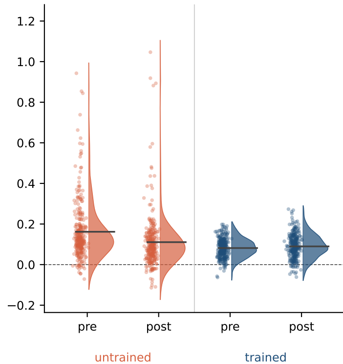
part-driven (part \rightarrow part) \Delta_{untrained}=-0.05 | \Delta_{trained}=+0.01
