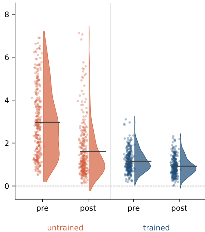
downward (whole \rightarrow part) \Delta_{untrained}=-1.36 | \Delta_{trained}=-0.23
