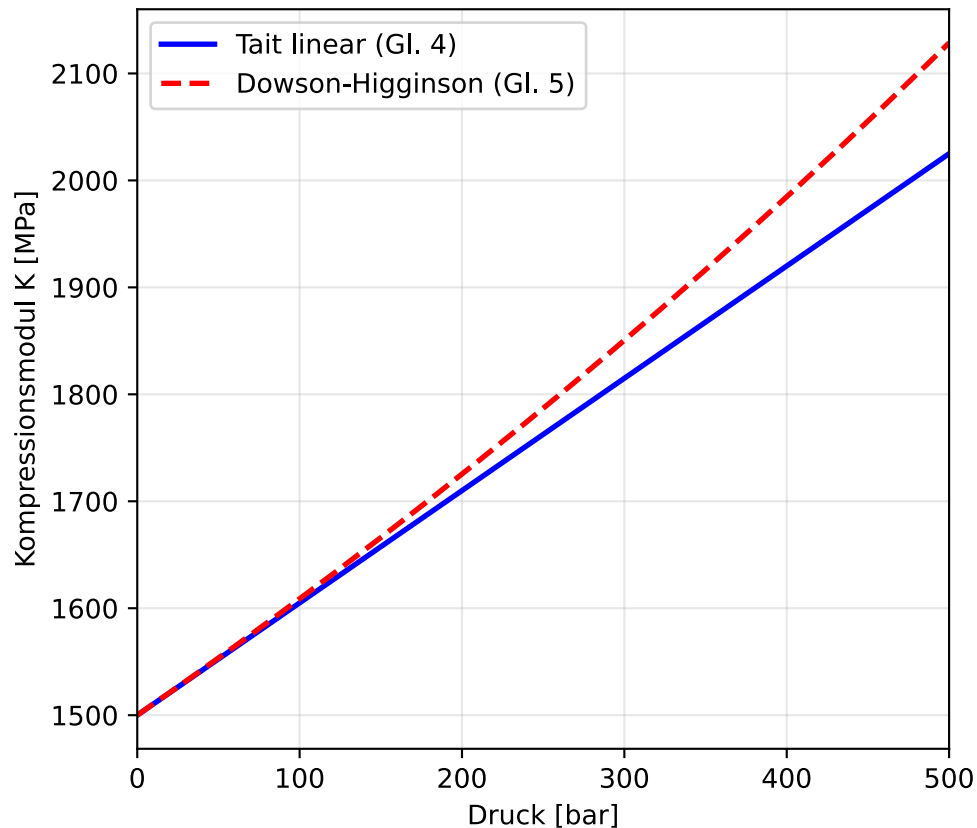
Tait vs. Dowson-Higginson
