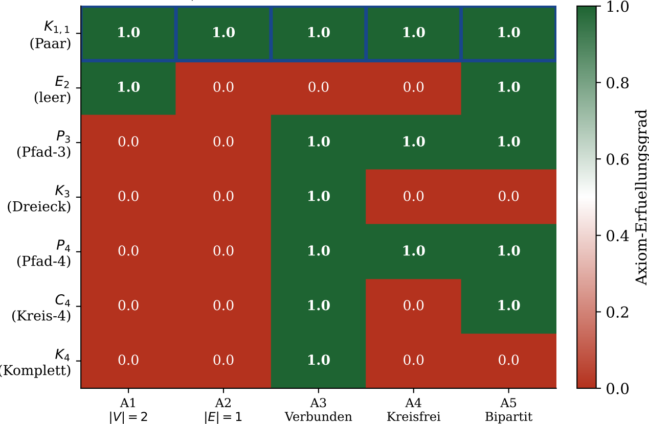
(a) Axiom-Erfuellungsmatrix ( K_{1,1} erfuilt alle Axiome maximal)
