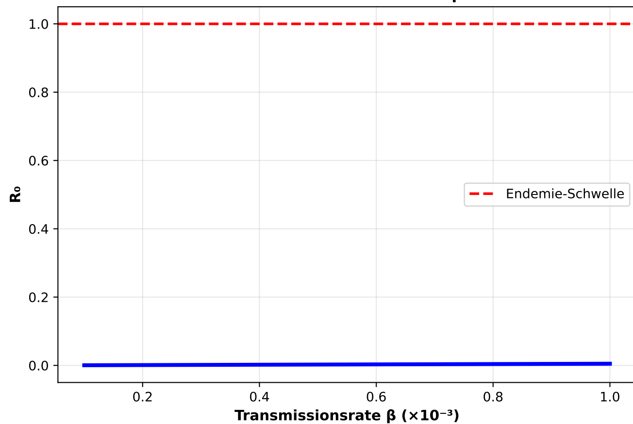
R_0 vs. Transmissionsrate \beta
