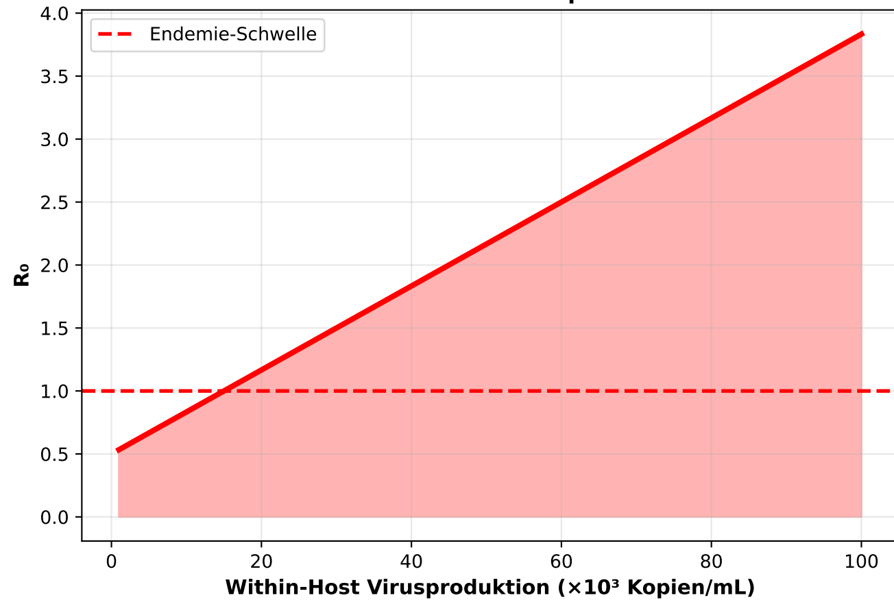
R_0 vs. Within-Host Replikation
