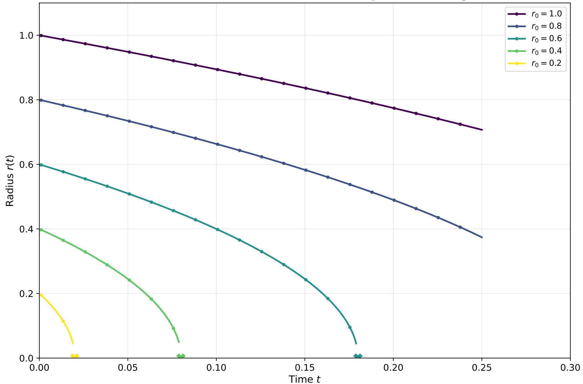
Deterministic Mean Curvature Flow: Sphere Shrinking
