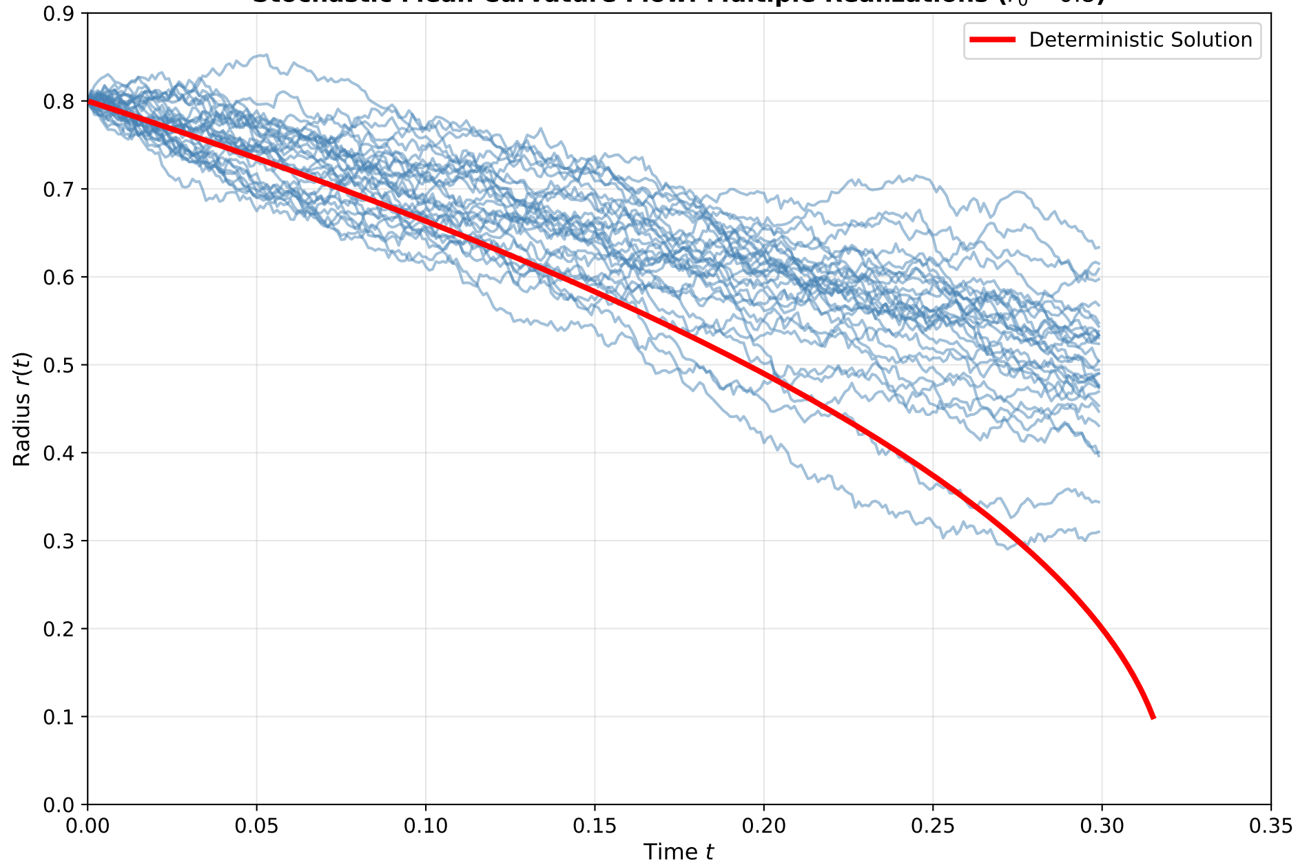
Stochastic Mean Curvature Flow: Multiple Realizations ( r_0 = 0.8 )
