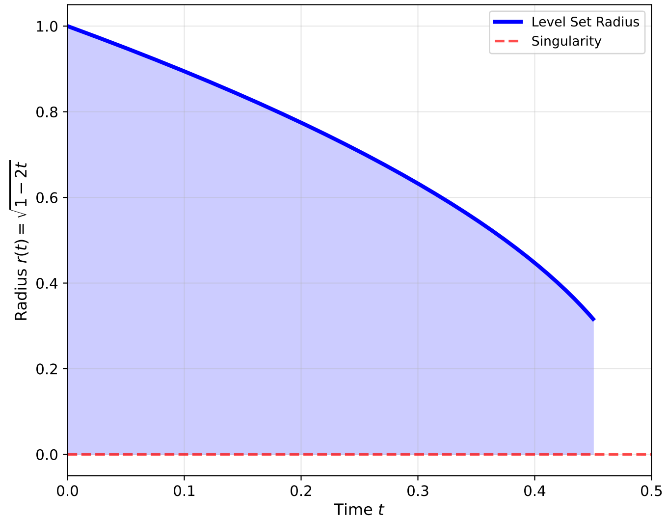
Level Set Radius vs. Time
