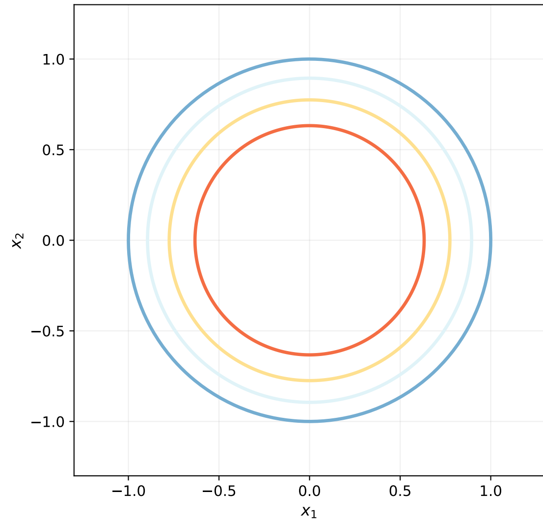
Deterministic Level Sets Evolution
