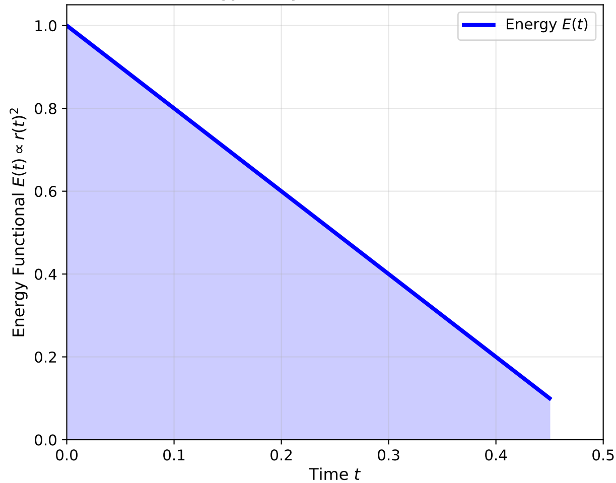
Energy Decay (Deterministic Case)
