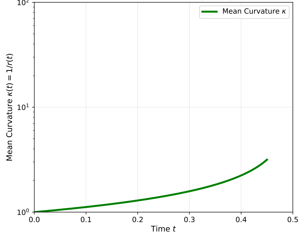
Curvature Growth to Singularity
