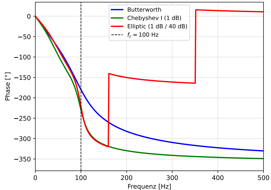
Phasengang
