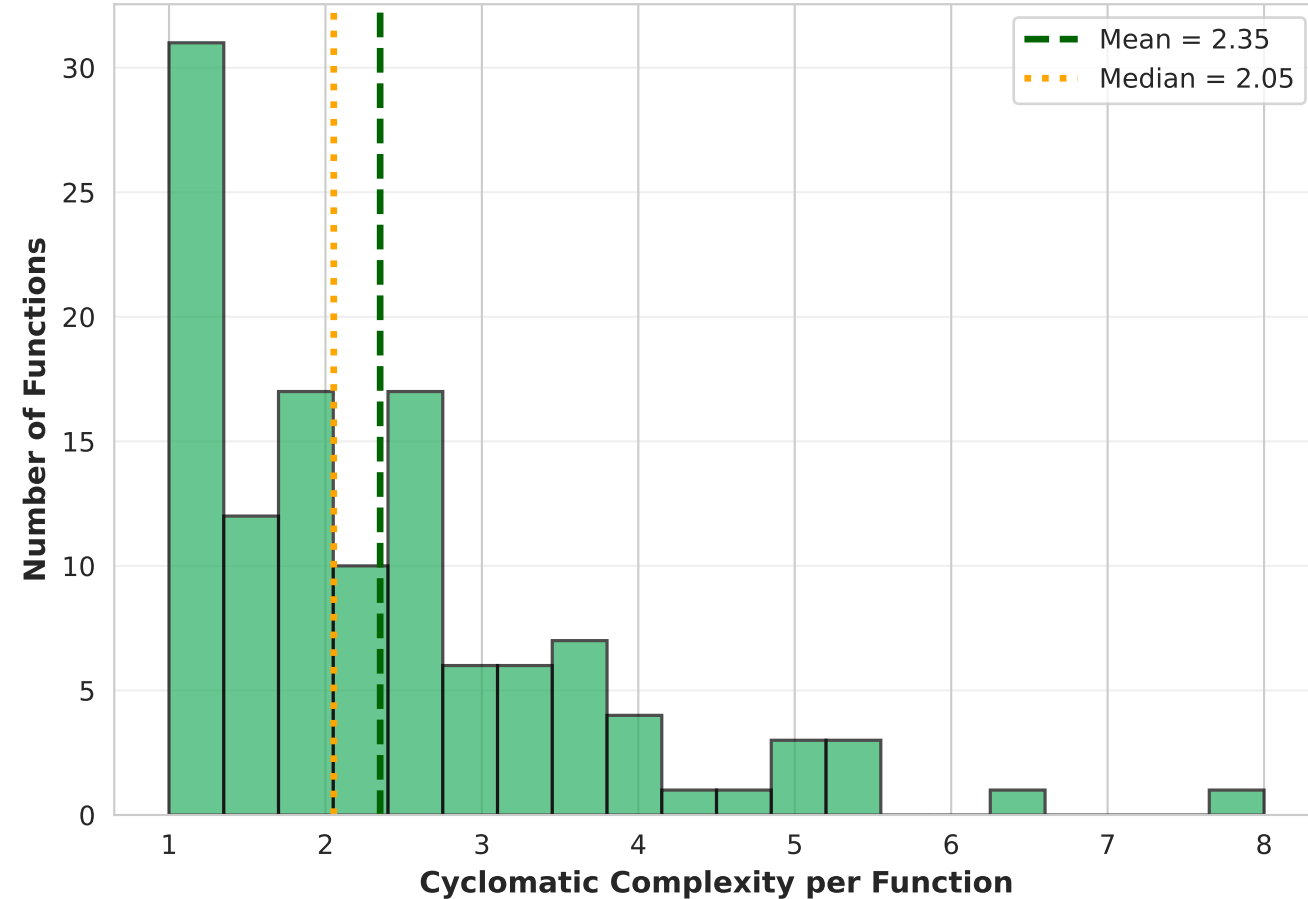
Decomposed System (120 functions, \mu=2.3 , \sigma=1.1 )
