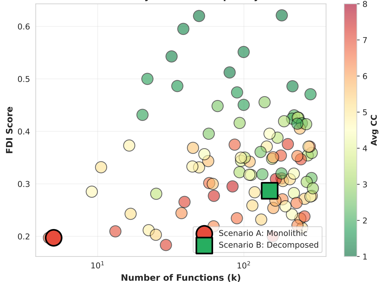
(a) FDI vs Function Count Color: Cyclomatic Complexity
