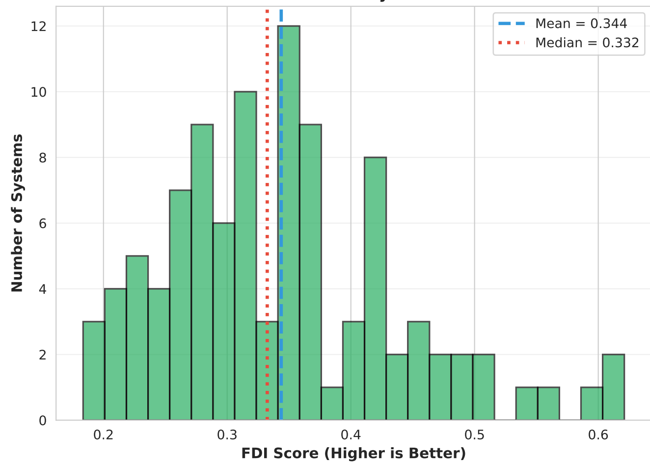
(b) Distribution of FDI Scores Across 100 Systems
