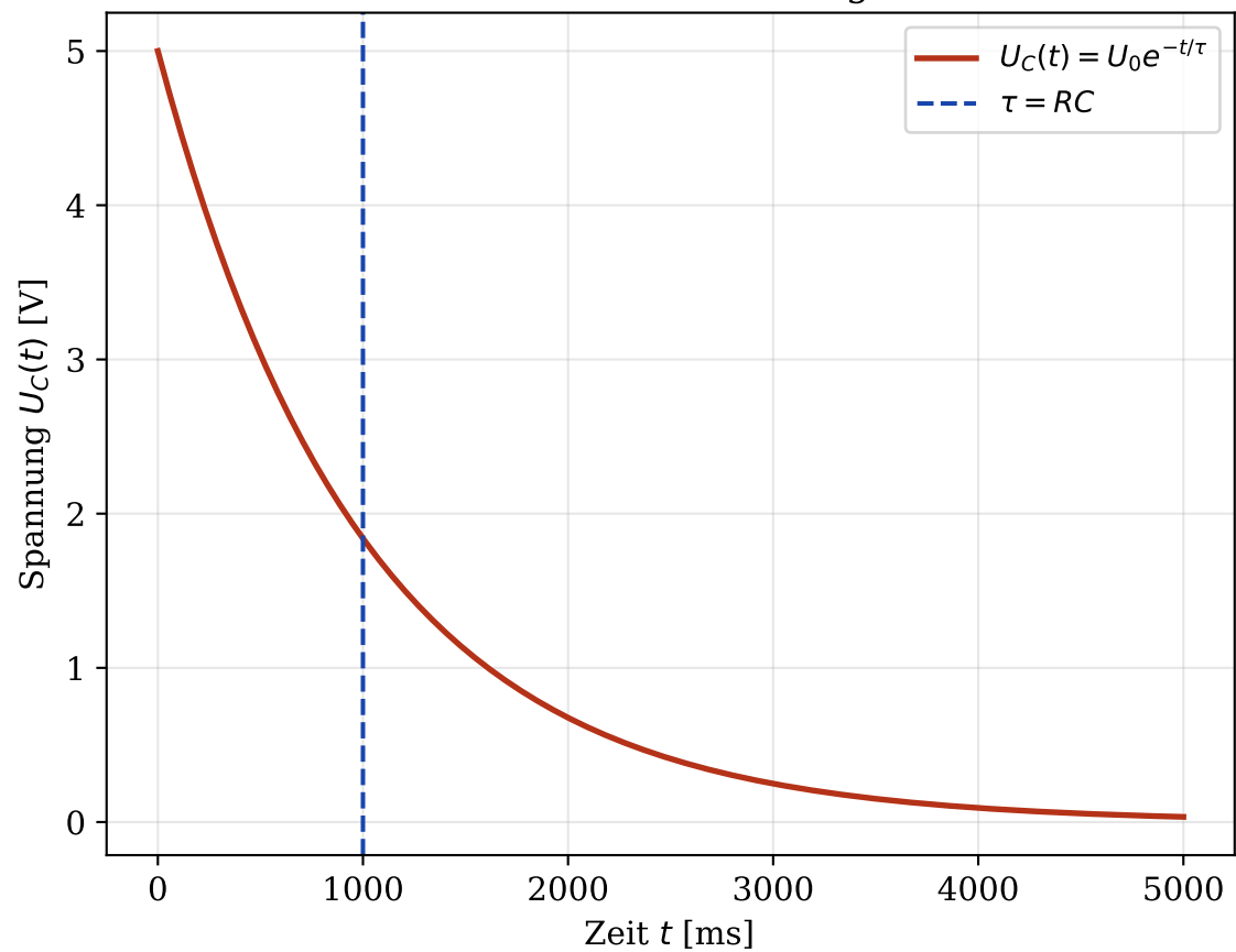
RC-Glied: Entladung
