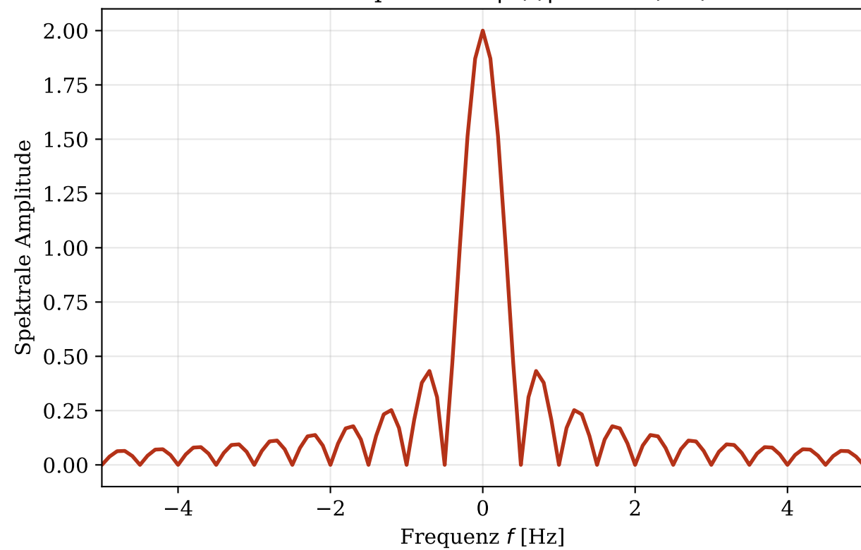
Fourier-Spektrum: |\hat{x}(f)| = T \operatorname{sinc}(\pi f T)
