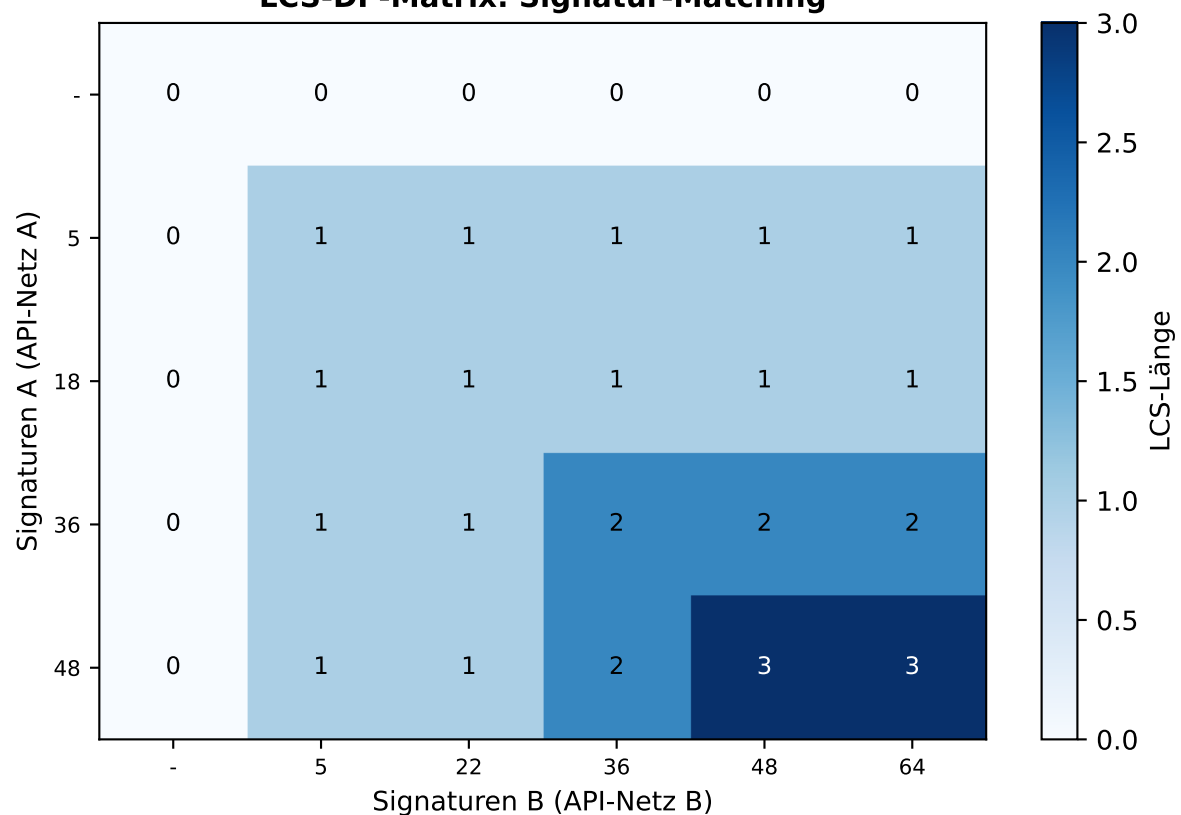
LCS-DP-Matrix: Signatur-Matching
