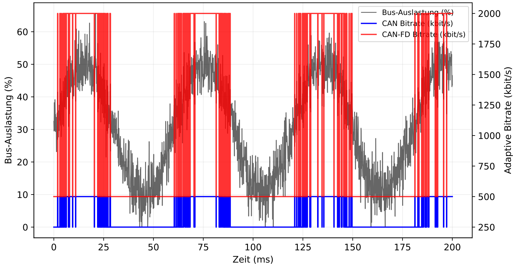
Adaptives Bitrate-Scheduling in Echtzeit
