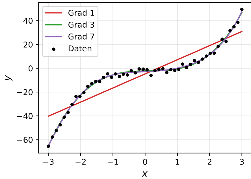
Polynominterpolation (NumPy)
