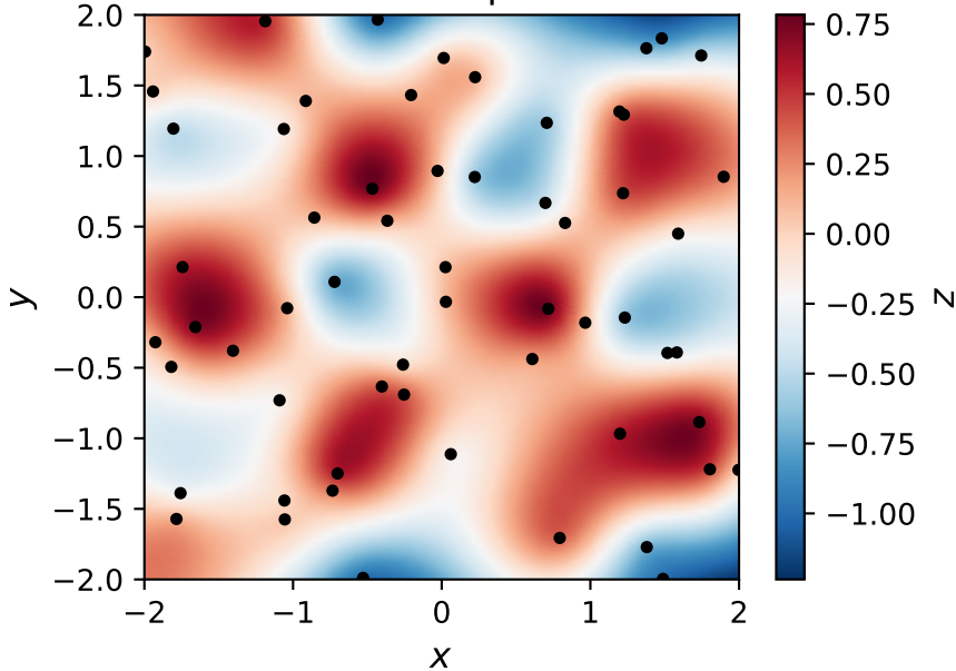
RBF 2D-Interpolation
