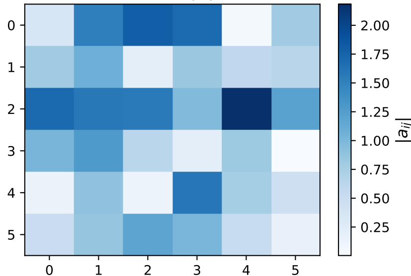
Matrix |A|
