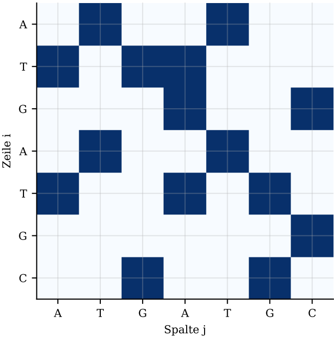
Deletion -C (Pos. 3) → 7×7 Matrix
