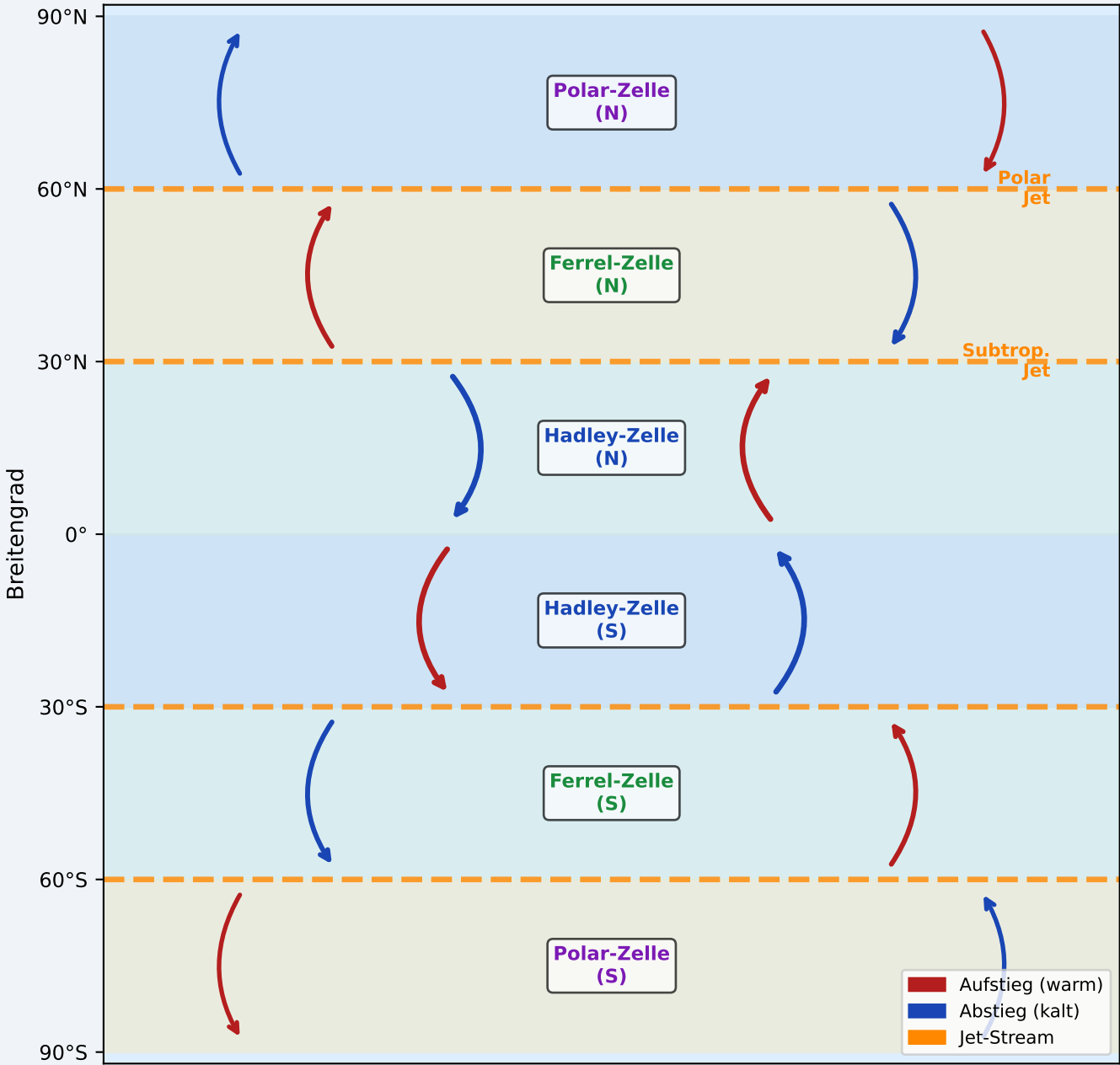
Meridionale Zirkulationszellen (Hadley, Ferrel, Polar)
