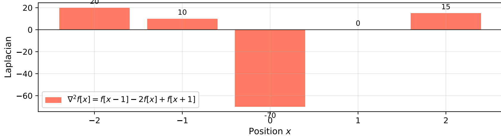
Diskrete Laplacian-Approximation \nabla^2 f[x]
