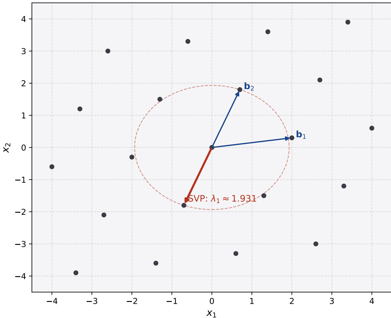
Shortest Vector Problem (SVP) in \mathbb{R}^2
