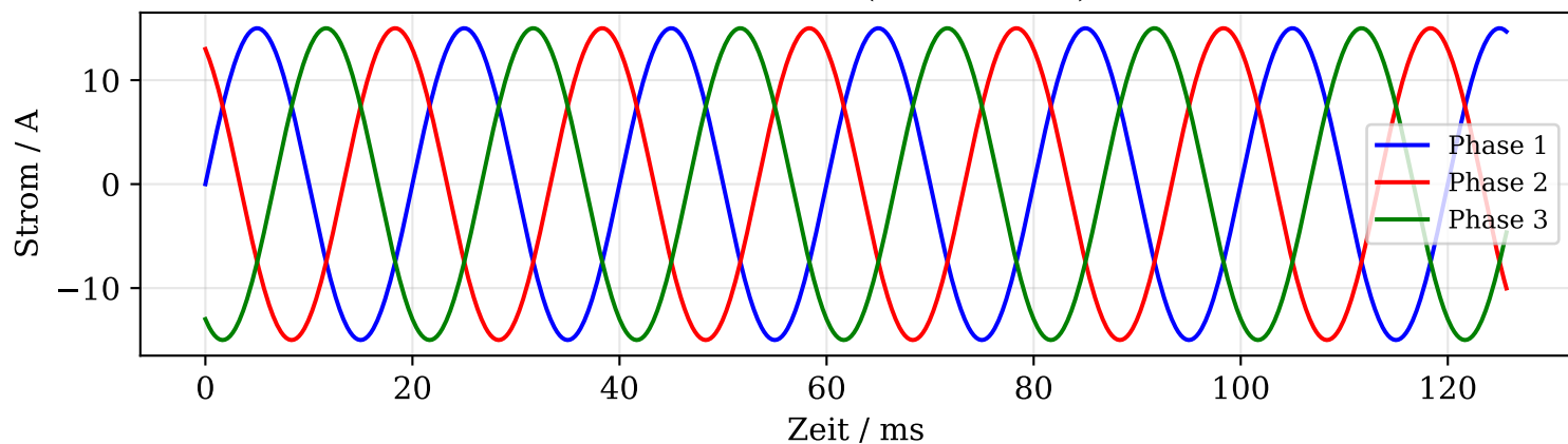
GaNius PFC (THD < 2%)
