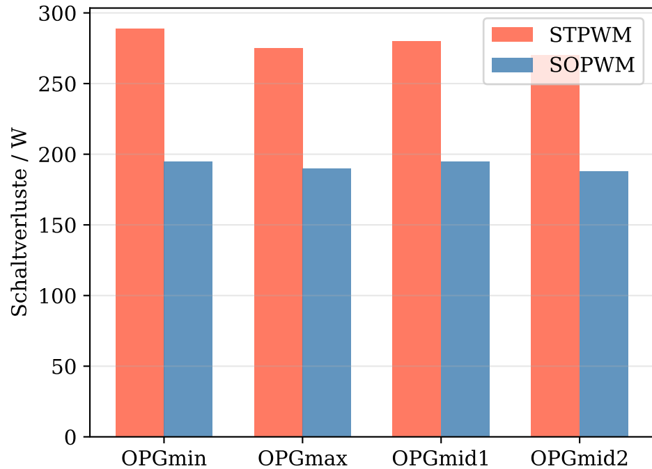
STPWM vs. SOPWM
