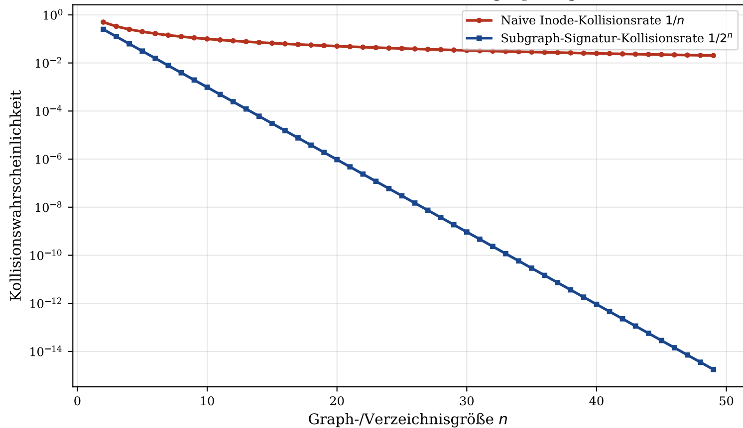
Kollisionsrate: Inode-Hash vs. Subgraph-Signatur
