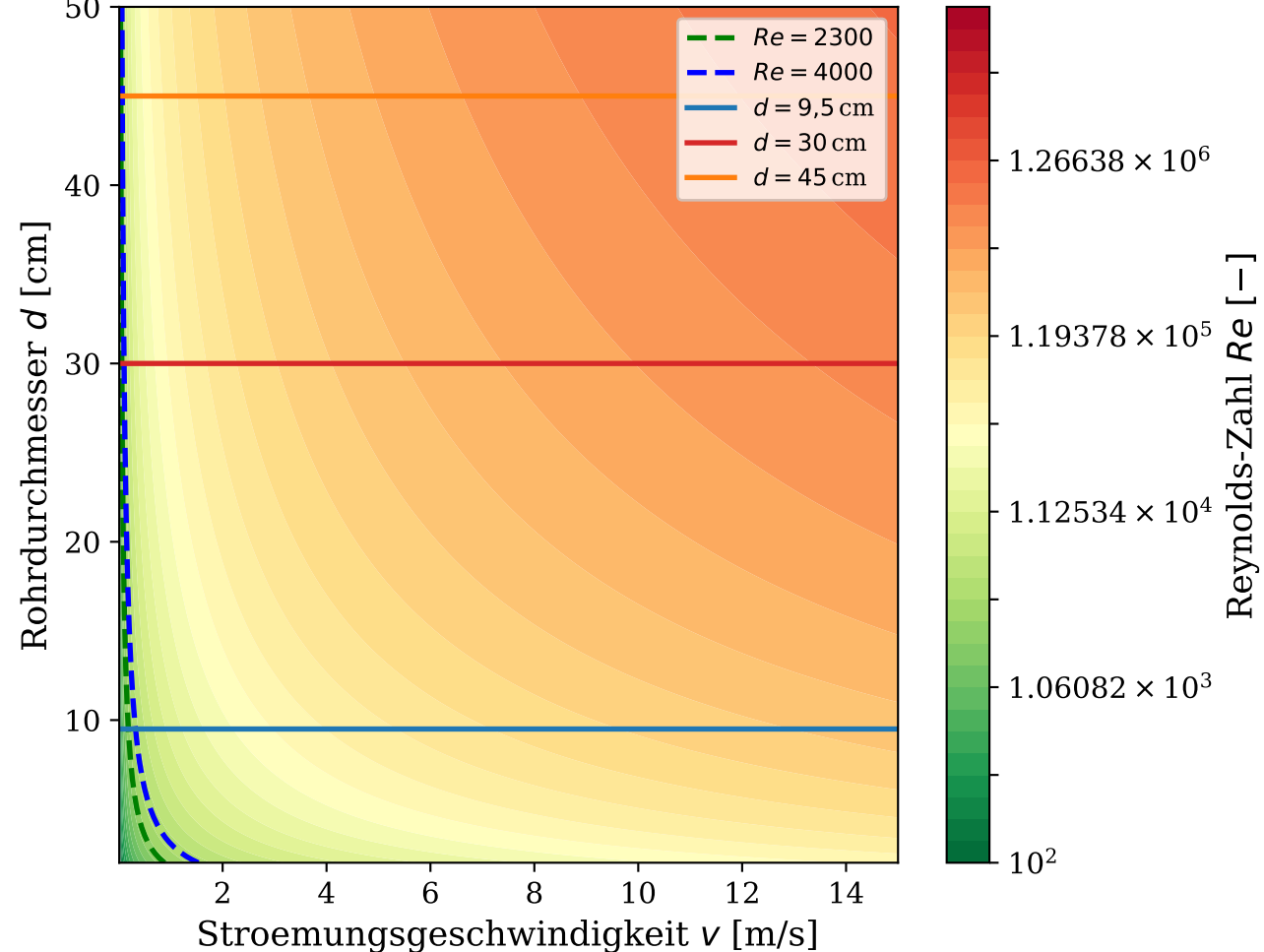
Stroemungsregime-Karte Re(v, d)
