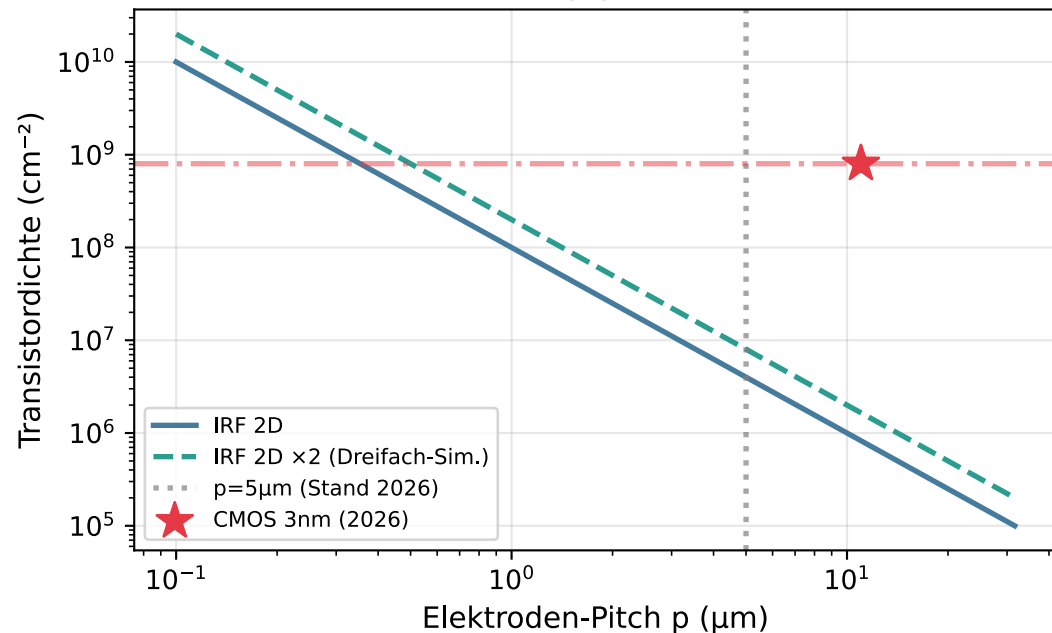
IRF-Transistordichte \rho(p) vs. CMOS-Referenz
