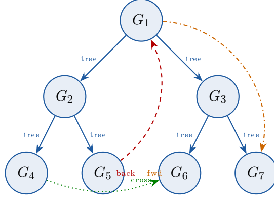
Abbildung 1: Schematic DFS forest on a meta-graph of seven graphs. Tree edges (solid blue) form the primary containment hierarchy. The back edge (dashed red, G_5 \rightarrow G_1 ) indicates circular containment. The cross edge (dotted green, G_4 \rightarrow G_6 ) reveals lateral structural similarity. The forward edge (dash-dot orange, G_1 \rightarrow G_7 ) encodes transitive containment.
