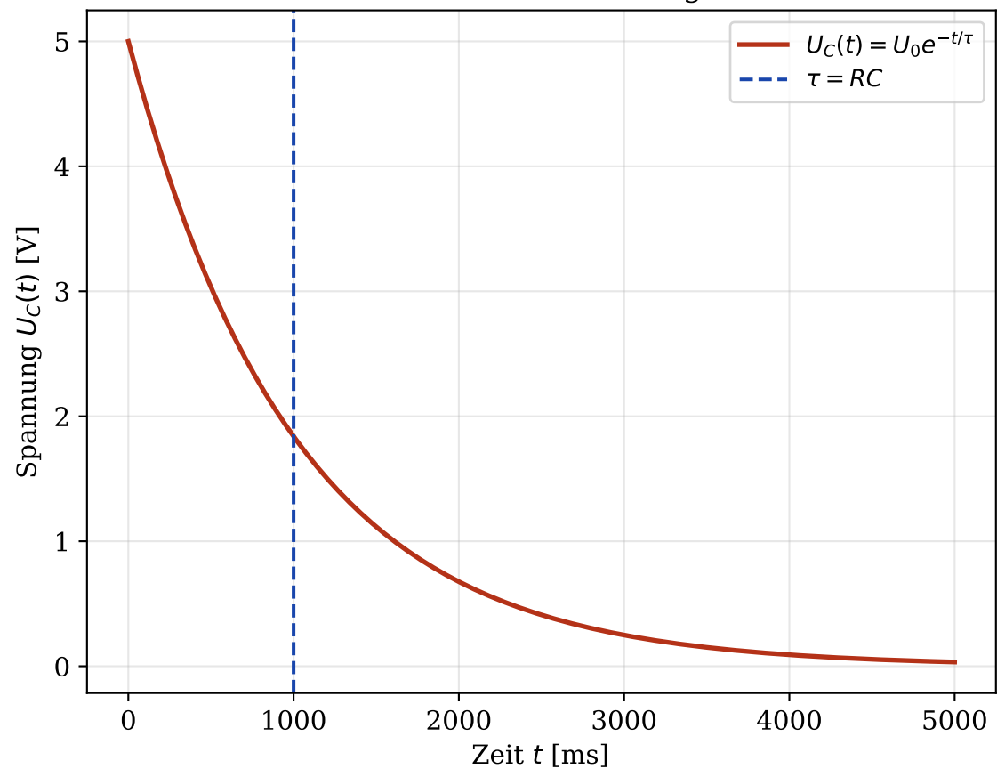
RC-Glied: Entladung
