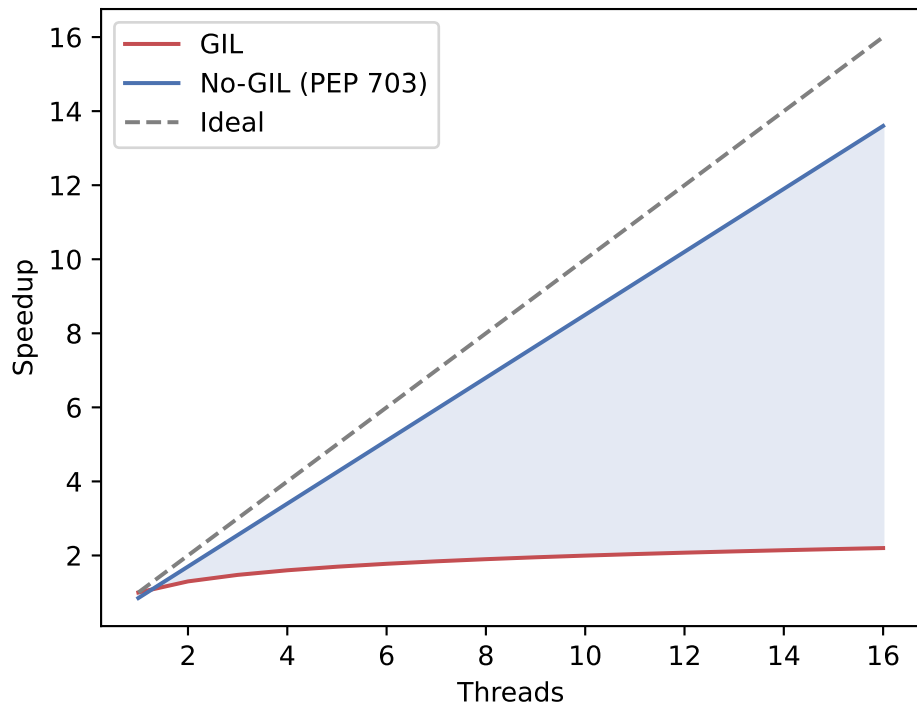
Speedup: GIL vs. No-GIL
