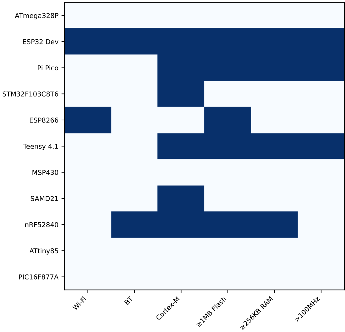
Feature-Matrix
