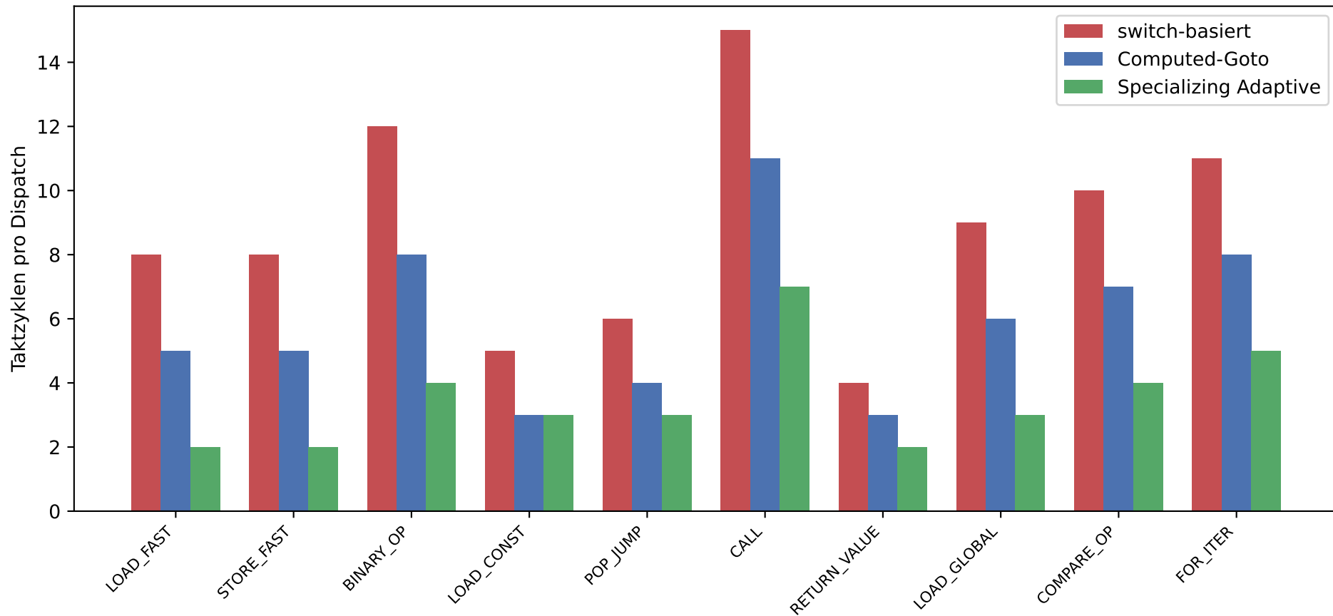
Opcode-Dispatch-Kosten: switch vs. Computed-Goto vs. SAI
