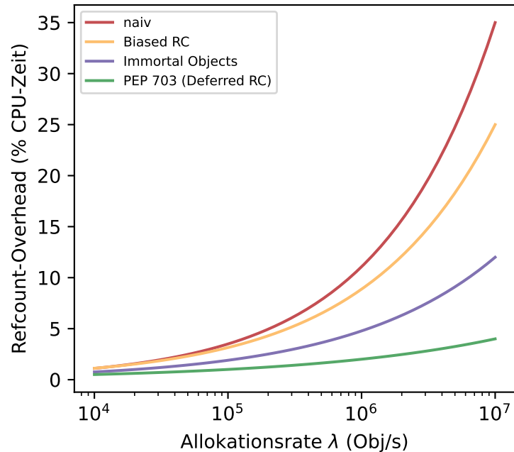
Recount-Overhead
