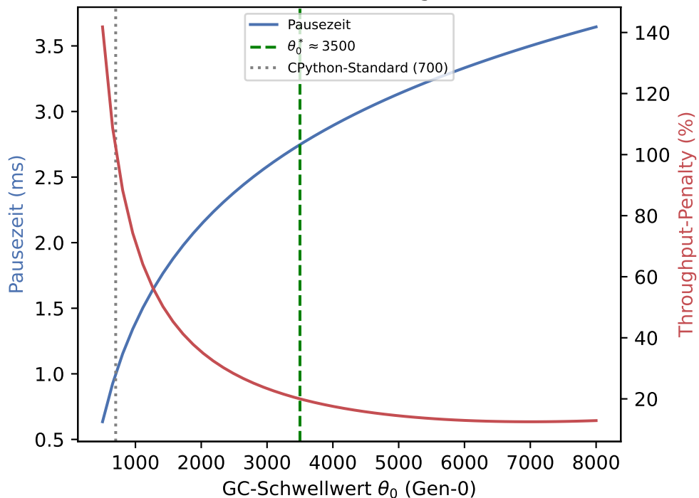
GC-Schwellwert-Tuning (Gen-0)
