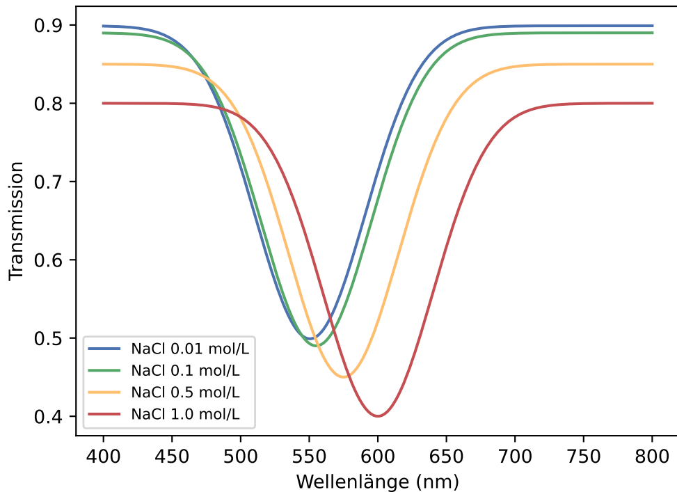
Plasmonen-Transmission
