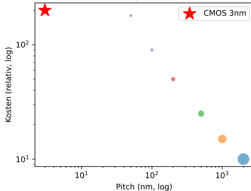
Technologie-Roadmap
