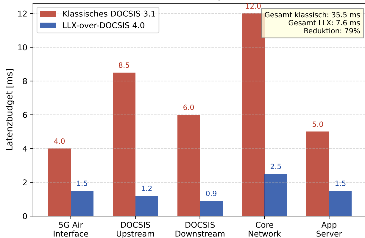
(a) End-to-End Latenzbudget: 5G + DOCSIS
