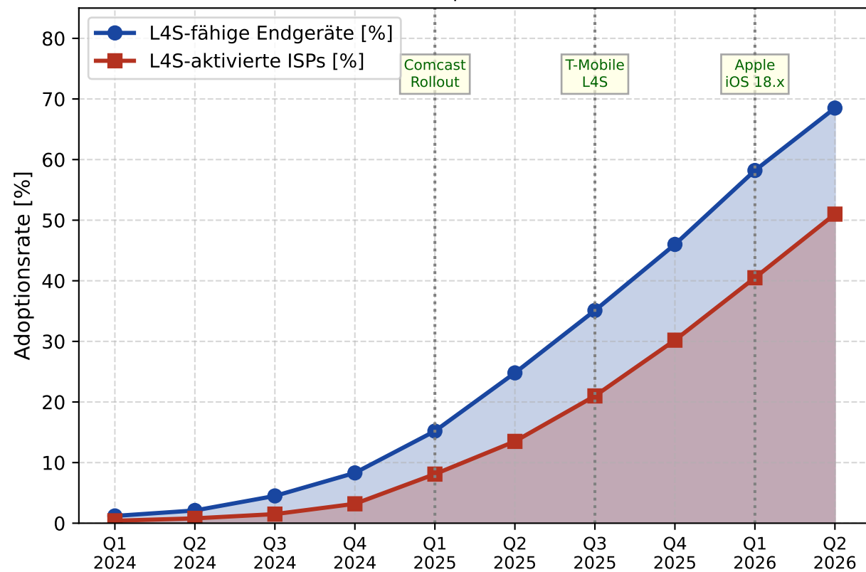
(a) L4S-Rollout-Adoptionskurve 2024-2026
