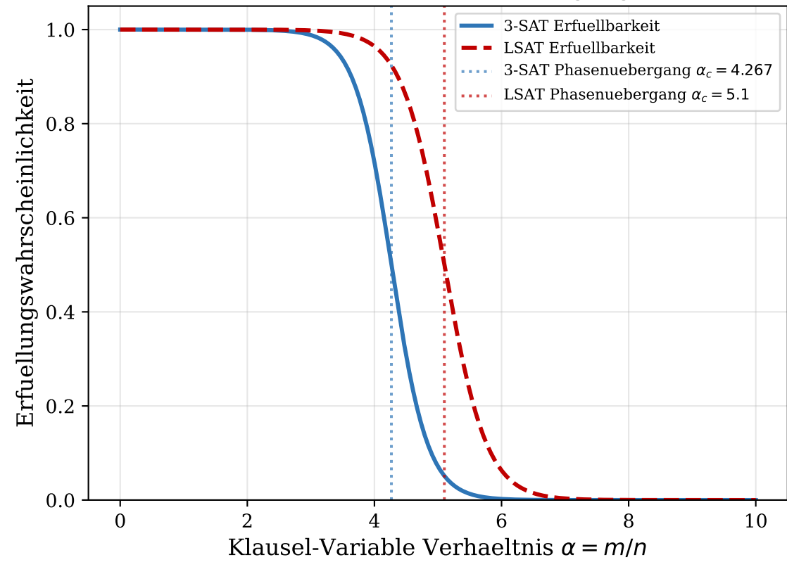
Abb. 7b: SAT-Phasenuebergang
