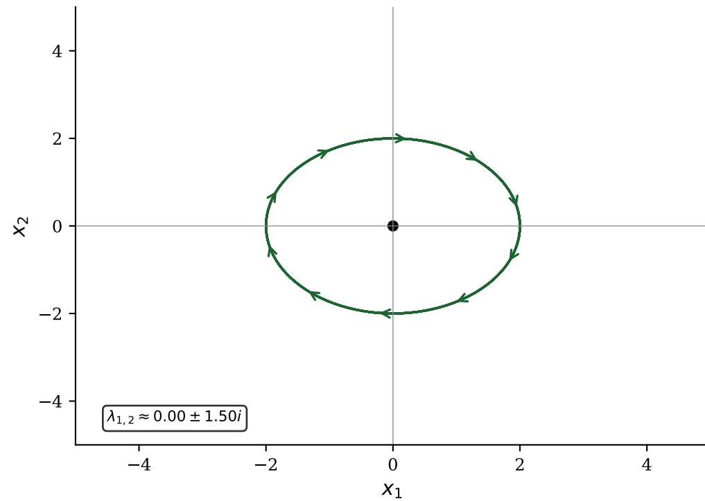
DP-II: Grenzstabile Depension \alpha^* = 0 , permanente Oszillation
