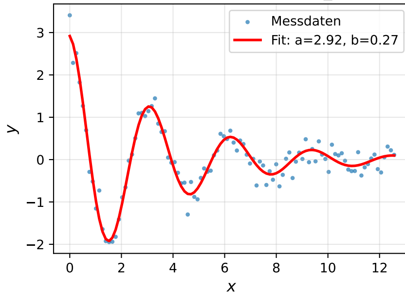
Kurvenanpassung (curve_fit)
