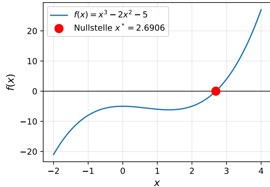
Nullstellensuche (Brent)
