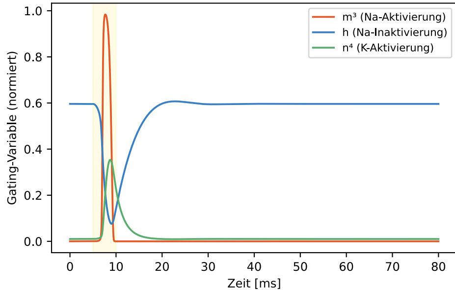
Gating-Variablen m^3 , h , n^4
