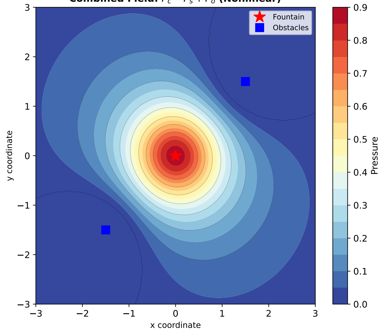
Combined Field: P_c = P_s + P_o (Nonlinear)
