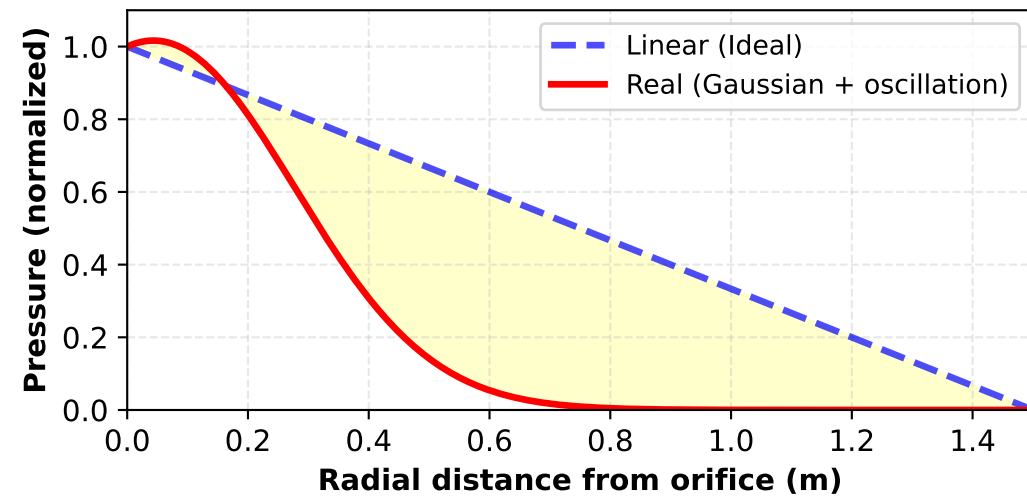
Radial Pressure Profile in Fountain
