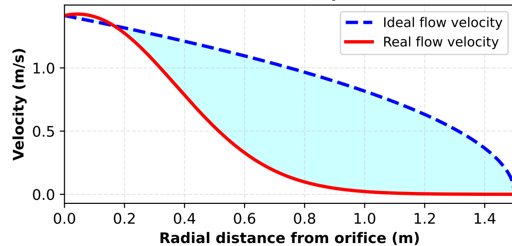
Fountain Water Velocity Distribution
