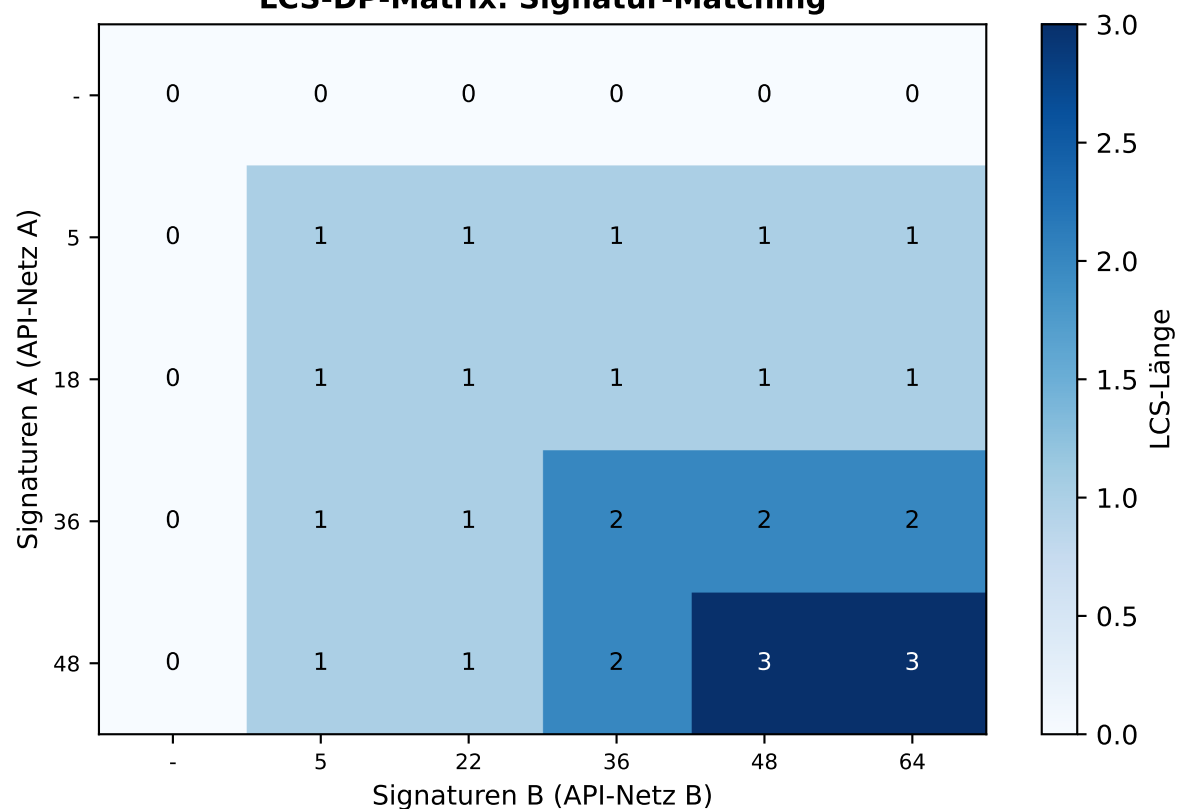
LCS-DP-Matrix: Signatur-Matching
