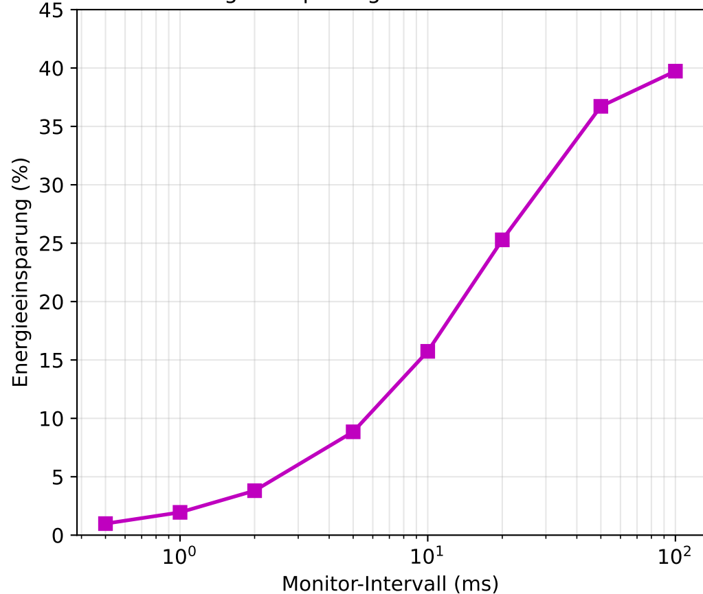
Energieeinsparung vs. Monitor-Intervall
