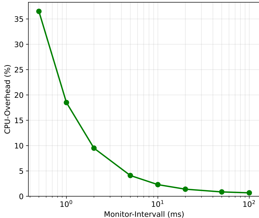
Monitoring-CPU-Overhead vs. Intervall
