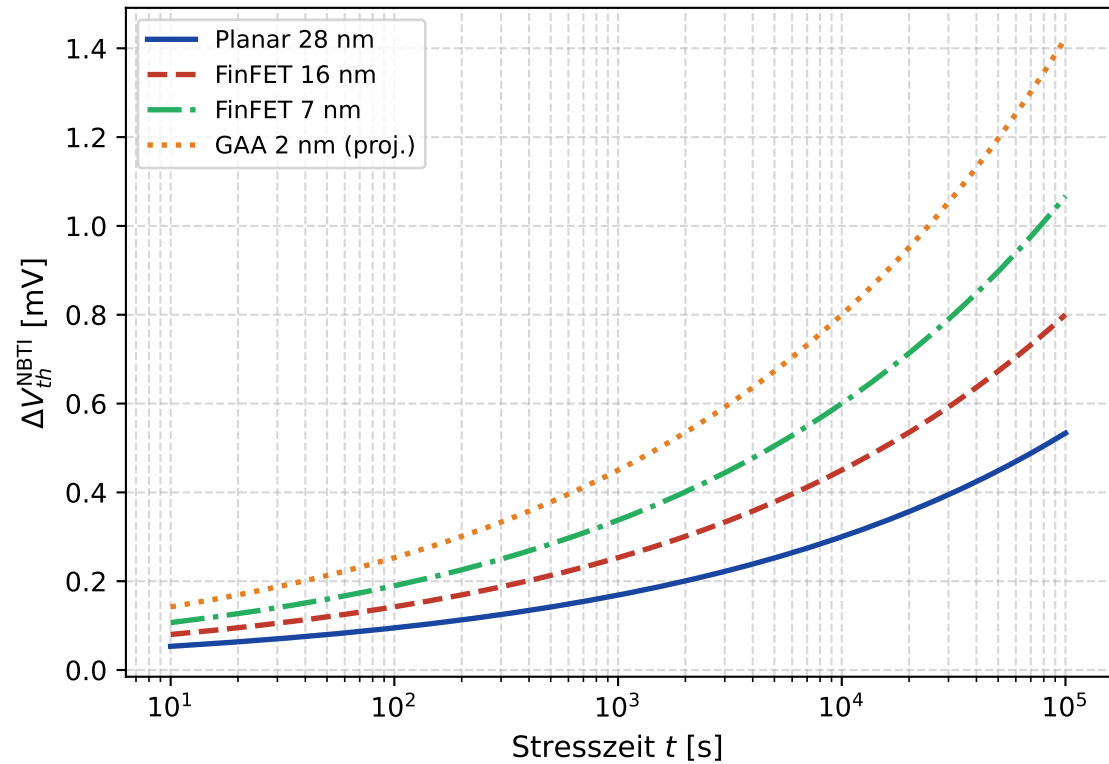
NBTI: Planar vs. FinFET vs. GAA
