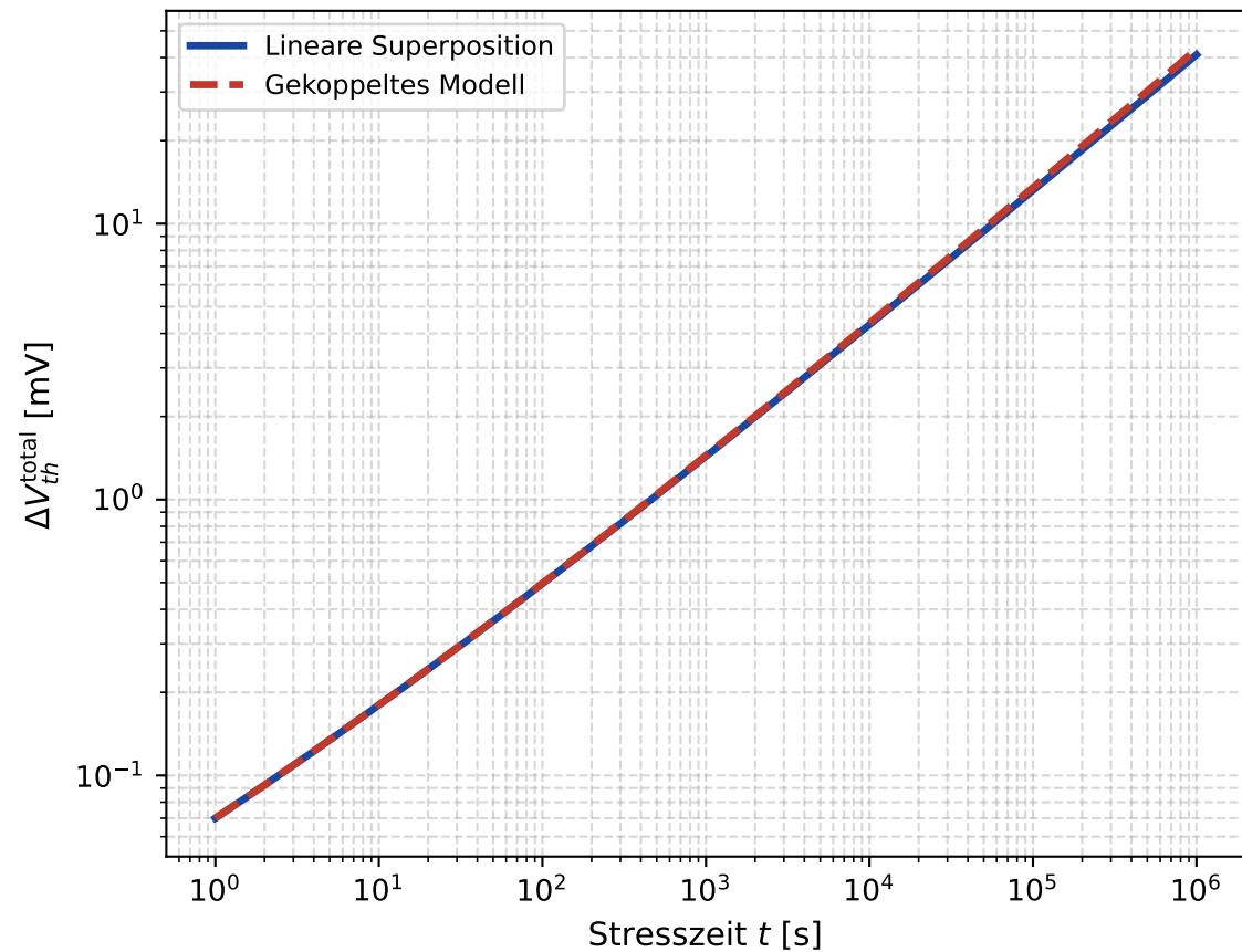
Kopplung vs. lineare Superposition
