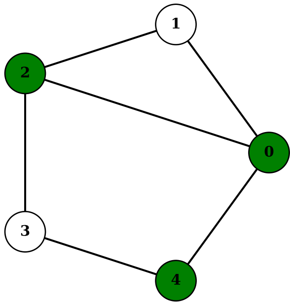
Independent Set
