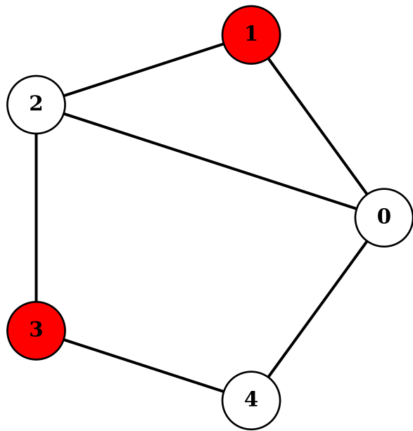
Vertex Cover
