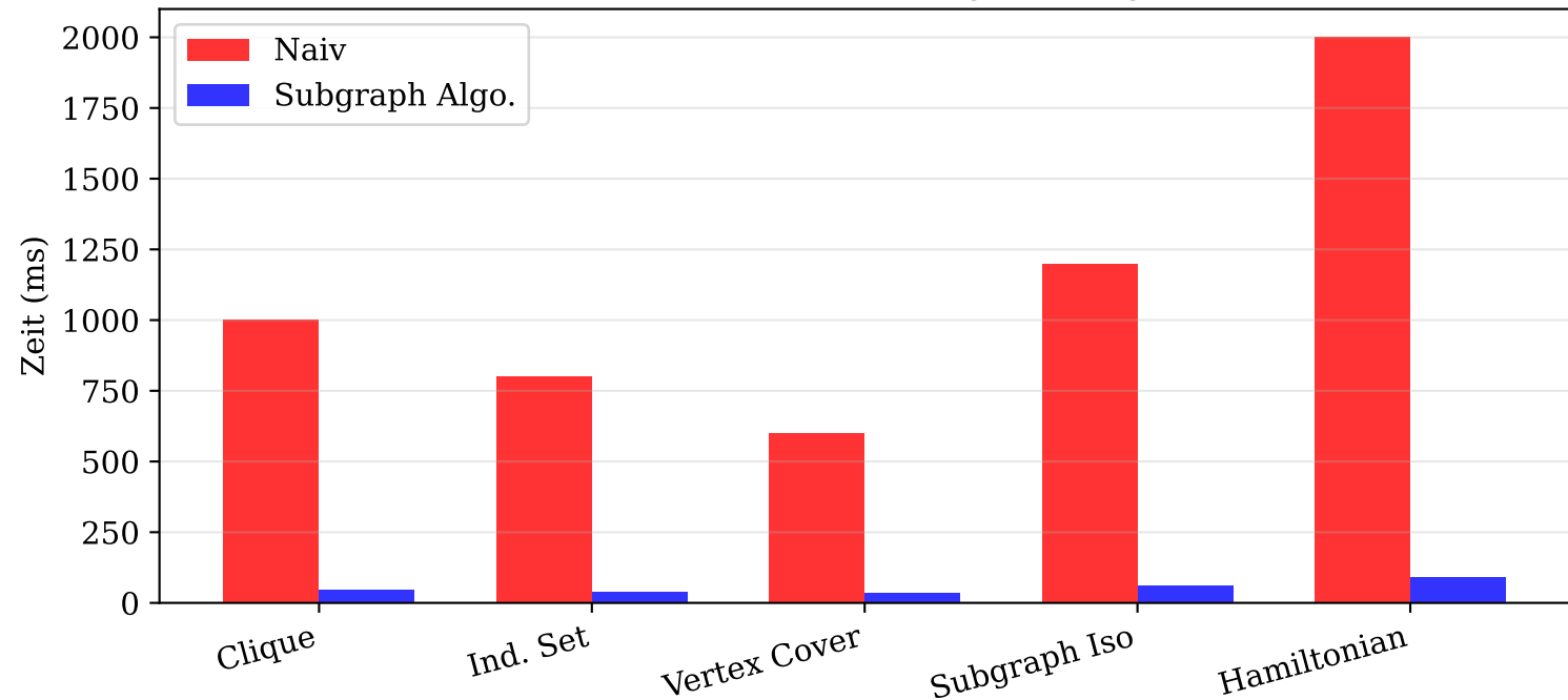
Graphprobleme: Naiv vs. Subgraph Algorithmus
